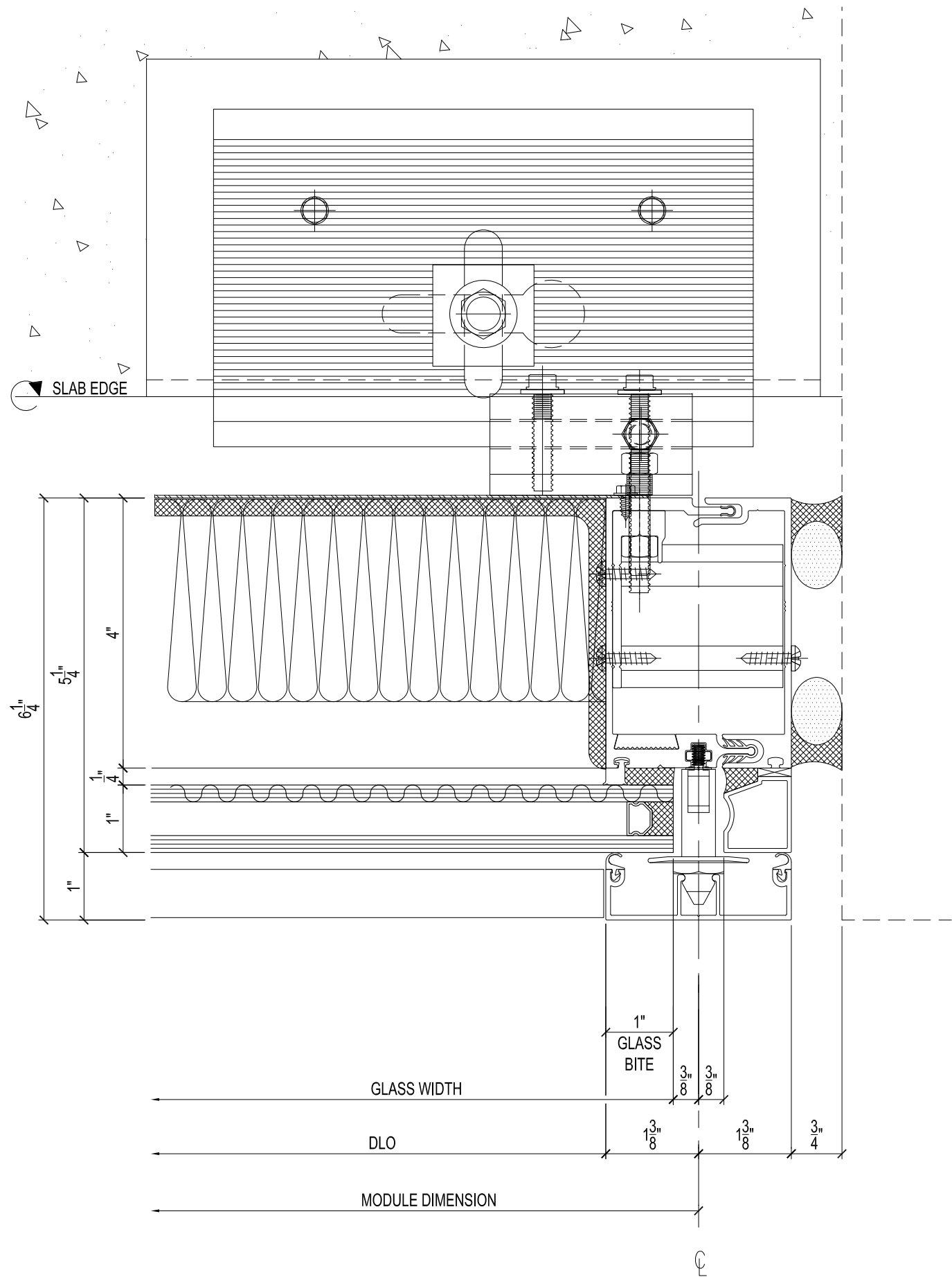
2 4 TYPICAL 2 3/4" JAMB MULLION DETAIL @ SPANDREL GLASS
