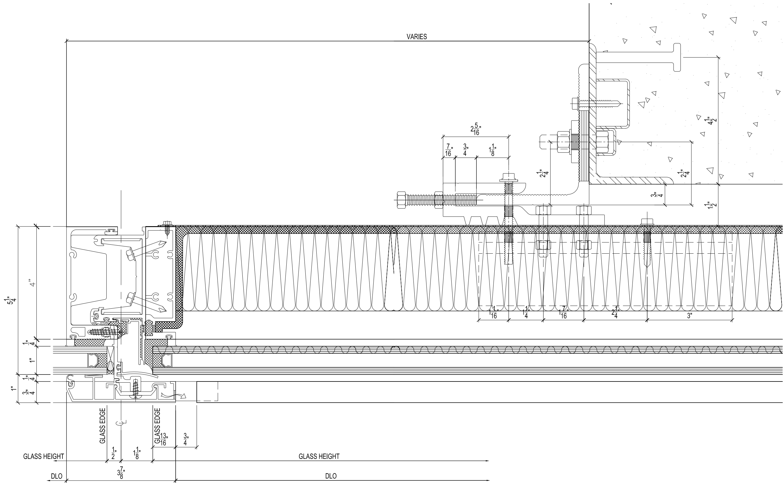
17 TYPICAL 3 7/8" STACK JOINT DETAIL
