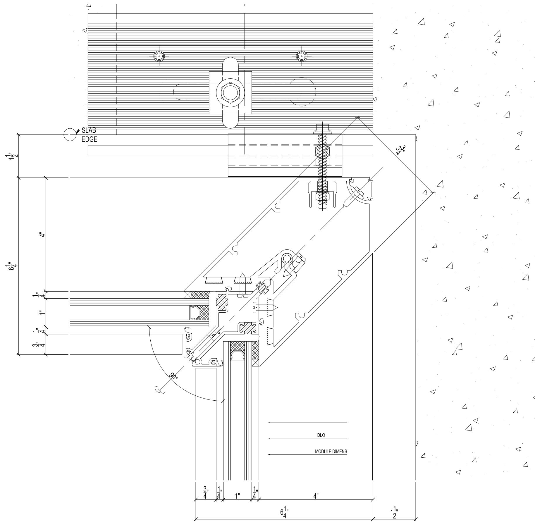
12 12 TYPICAL 90° CAPTURED INSIDE CORNER MULLION @ ANCHOR DETAIL
